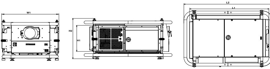
Projector Dimensions
